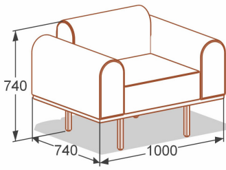
NOD single seater lounge
